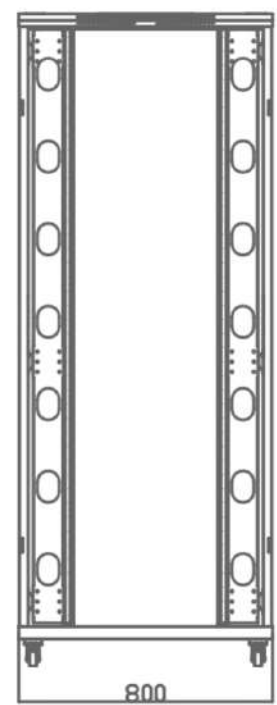
Back (Without door)
