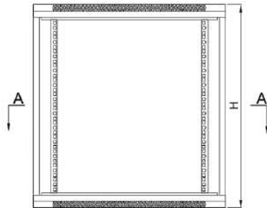
Front(without front door)
