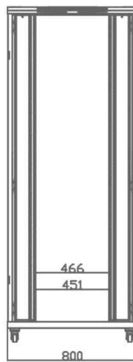
Front (Without door)
